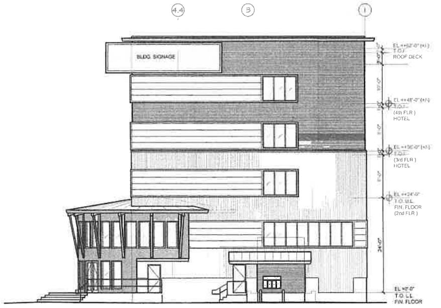
PROPOSED SOUTH ELEVATION SCALE: 1/8" = 1'-0"
